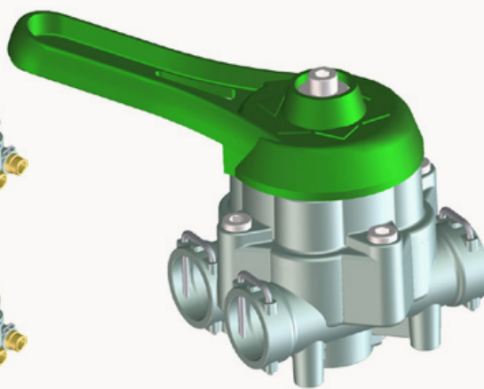
174.206.9 8P - 4 outlets selected one by one or in pairs - Green lever
