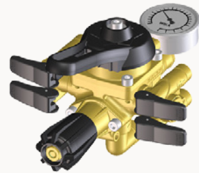
KR: 4 outlets version assembled with M172 valves
