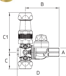
62.627.10 (Ø18)
