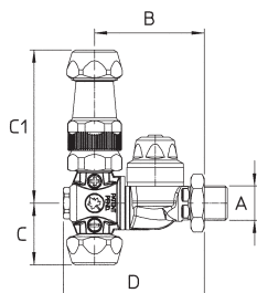
62.627.9 (Ø18) 62.627.12 (Ø15)
