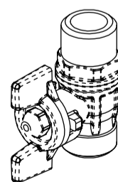
VARIANTE STANDARD STANDARD MODEL
